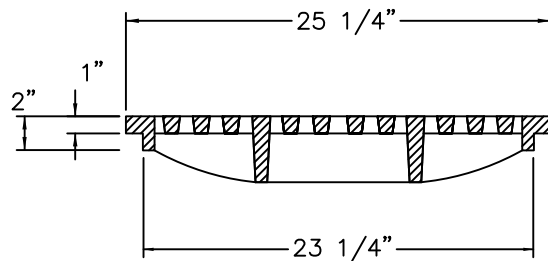
COVER
