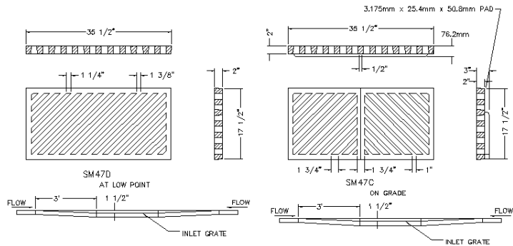
DEPRESSION IN FLOW LINE AT INLET CONSTRUCTION DETAILS
