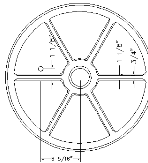
BOTTOM VIEW OF COVER CATCH BASIN AND MANHOLE COVER
