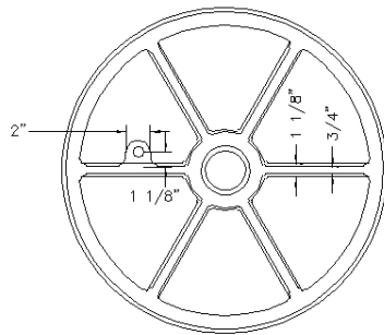
BOTTOM VIEW OF COVER
