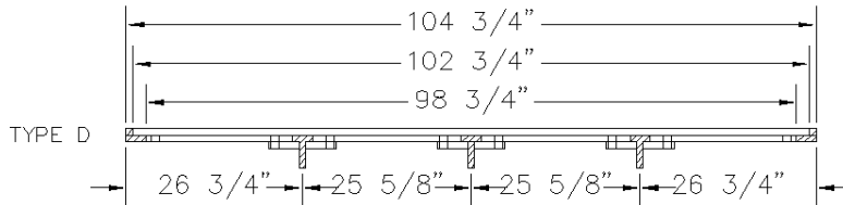
PLAN - TYPE B, C, & D FRAMES
