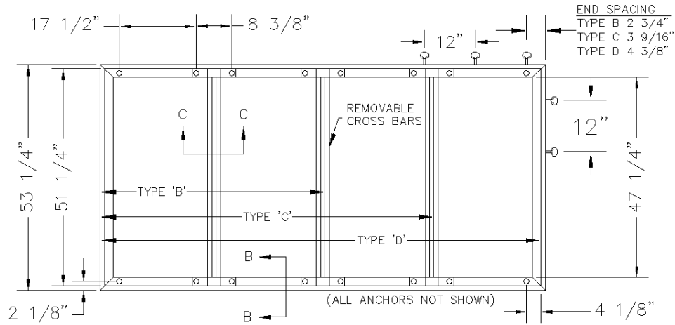
PLAN - TYPE B, C, & D FRAMES
