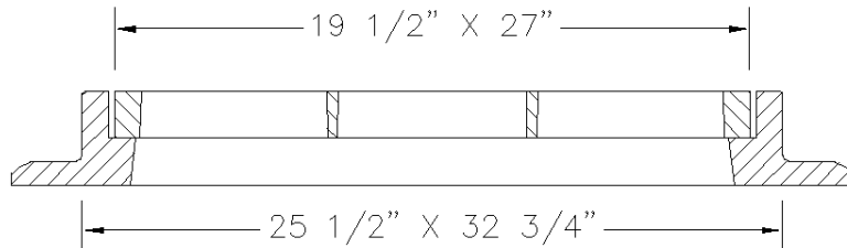
SMU-3110 FLAT GRATE
