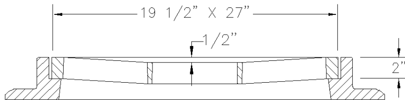
SMU-3100 CONCAVE GRATE
