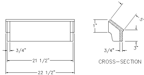
GRATE (BOTTOM VIEW)
