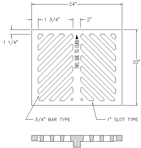
GRATE (SIDE VIEW)
