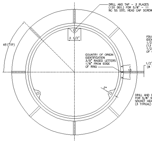
MANHOLE RING - PLAN
