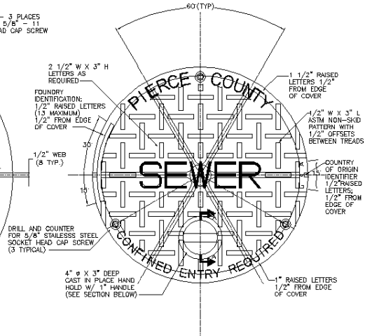
MANHOLE COVER - PLAN
