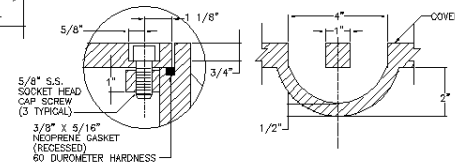
LOCKING BOLT - DETAIL HANDHOLE - SECTION A
