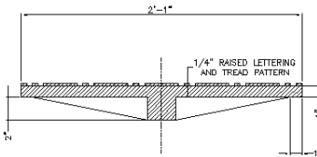
MANHOLE COVER - SECTION
